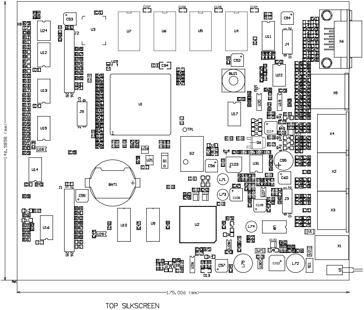
Figure B.6: Motherboard
