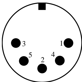
Figure 3.12: Packet-Radio connector (5-PIN DIN)
