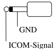
Figure 3.6: ICOM plug
