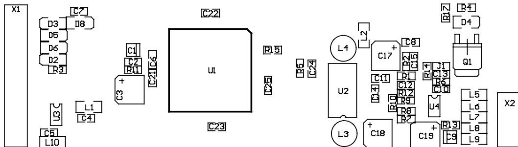
Figure 3.8: The DSP-Module.
