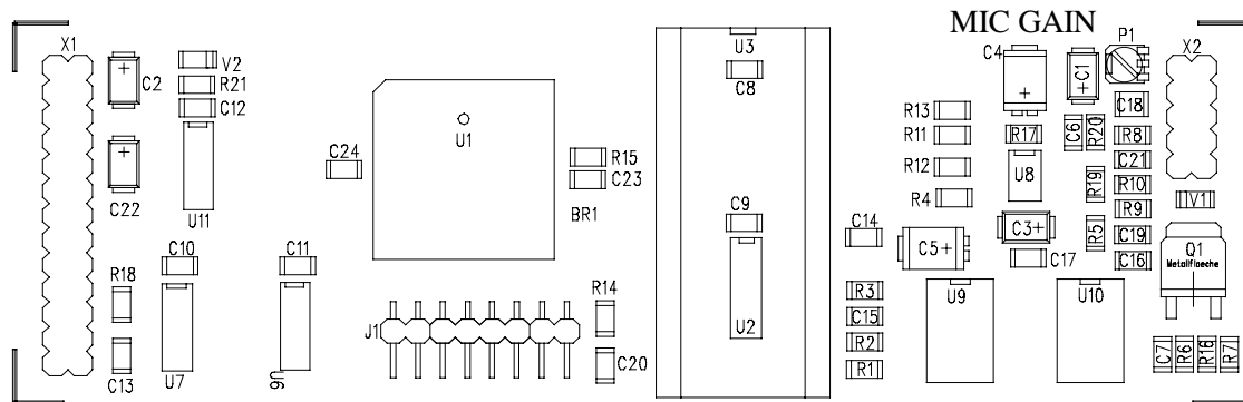
Figure 3.11: The 9k6-Module.
