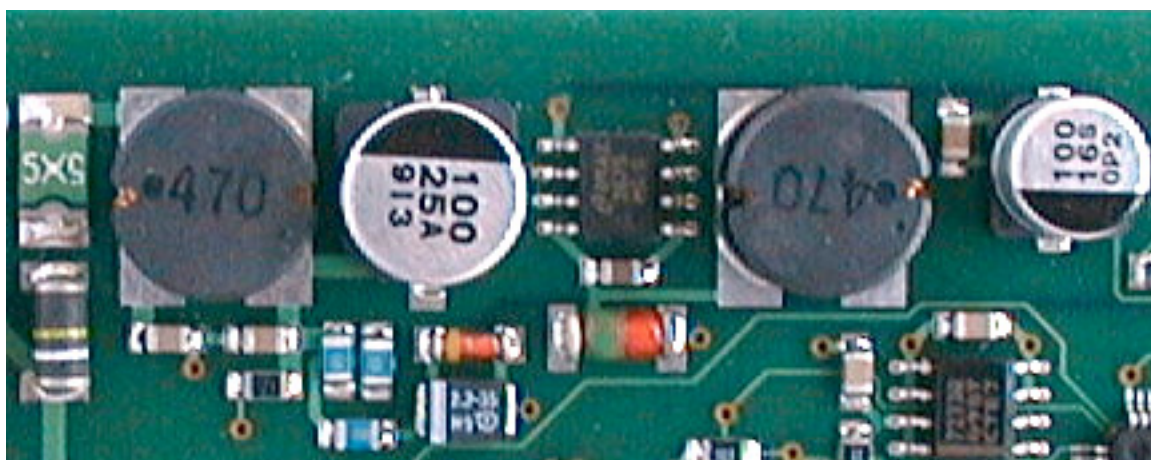
Figure 15.6: The PTC-IIpro switch-mode power unit.
