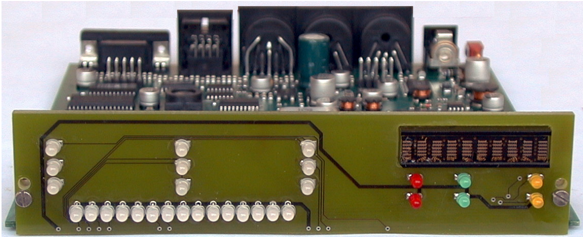
Figure 4.2: The PTC-IIpro front panel
